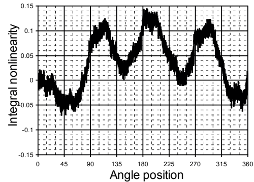
Fig. 15: Typical integral nonlinearity
