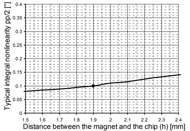
Fig. 30: Accuracy Vs Distance
