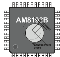
Fig. 24: Magnet displacement. Magnet is placed above the AM8192B.
