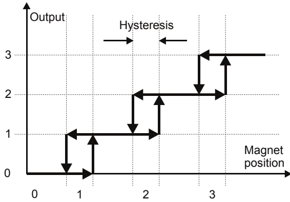
Fig. 9: Hysteresis
