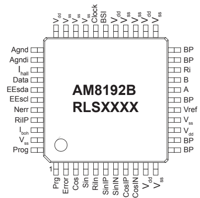
Fig. 1: Pin description for AM8192B
