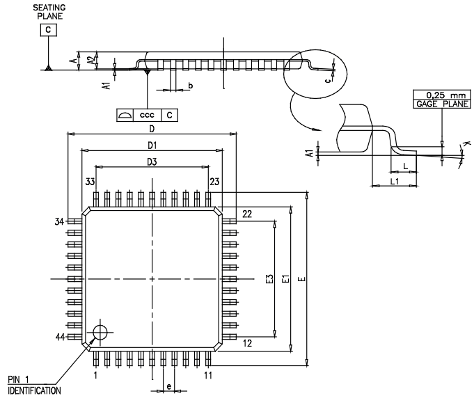
Fig. 34: LQFP44 package dimensions
