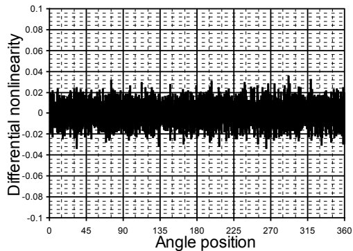
Fig. 14: Typical differential nonlinearity
