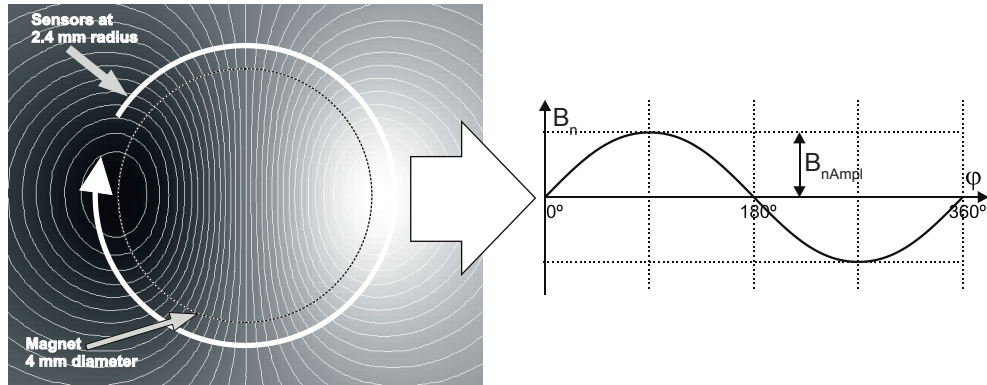
Fig. 18: Distribution of B_n and its modulation if the magnet is rotated through 360°
