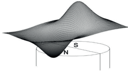
Fig. 17: Distribution of the perpendicular component of B
