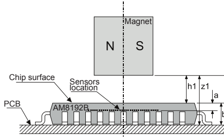
Fig. 21: Magnet placed above the AM8192B
