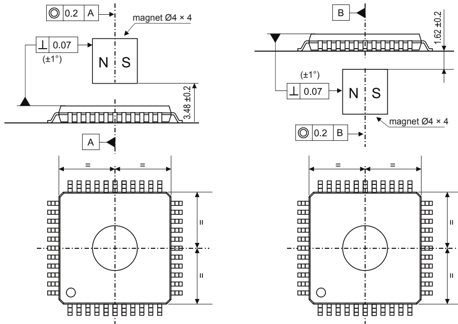
Fig. 23: Mounting instructions
